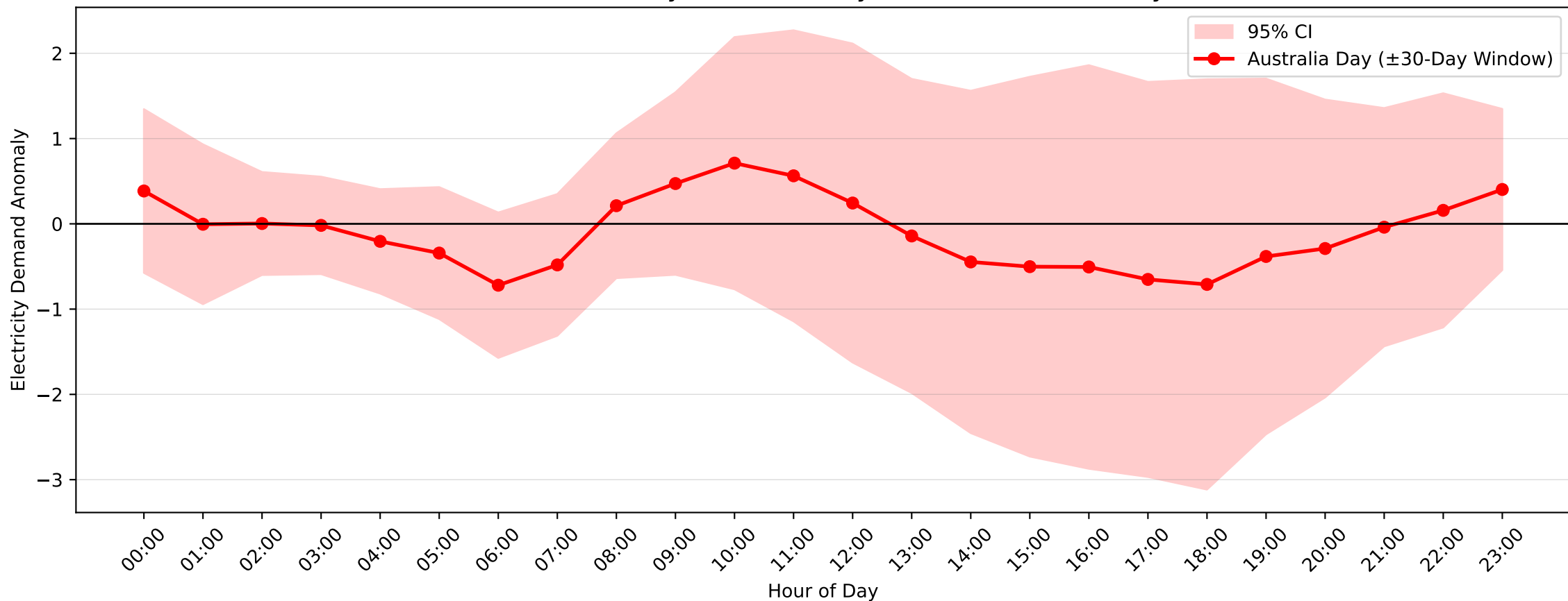
Umina Demand Anomaly: Australia Day (2004–2017, \pm 30 -Day Window)
